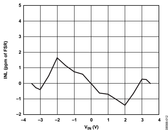
Figure 12. INL (Gain = 1)
