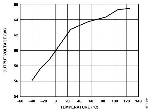
Figure 14. Offset Error (Gain = 1, Chop Disabled)
