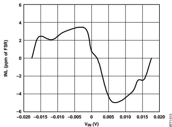
Figure 13. INL (Gain = 128)
