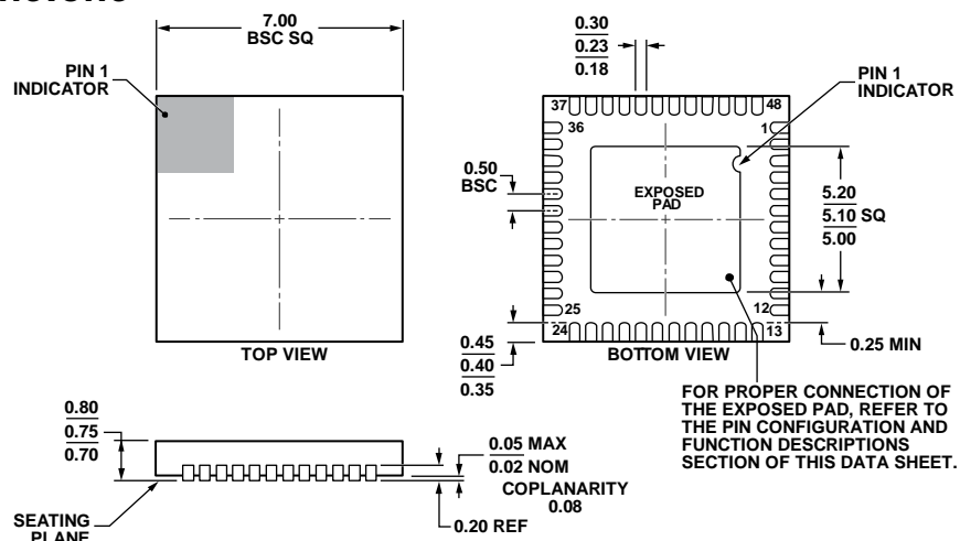
Figure 37. 48-Lead Lead Frame Chip Scale Package [LFCSP] 7 mm × 7 mm Body and 0.75 mm Package Height (CP-48-4)
