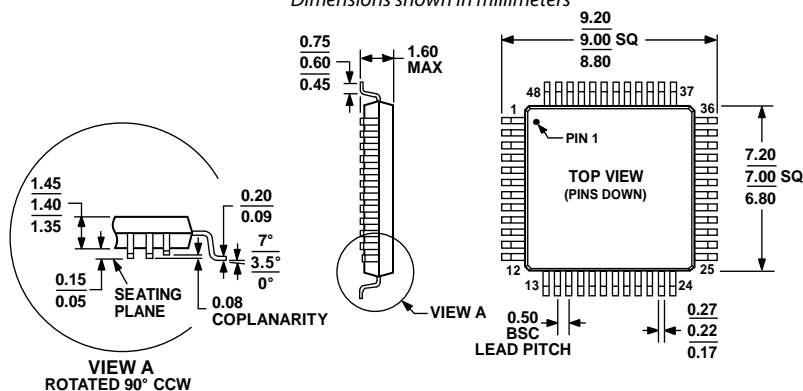
Figure 38. 48-Lead Low Profile Quad Flat Package [LQFP] (ST-48)
