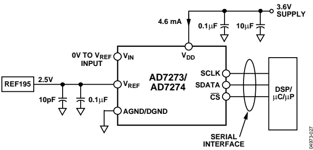
Figure 27. AD7273/AD7274 Typical Connection Diagram
