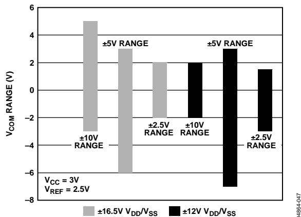
Figure 37. Common-Mode Range for V_{CC} = 3\text{ V} and REFIN/OUT = 2.5\text{ V}
