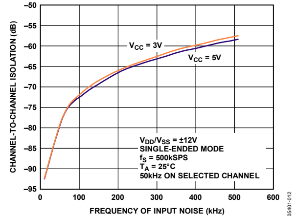
Figure 14. Channel-to-Channel Isolation
