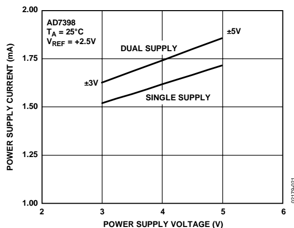
Figure 21. AD7398 Supply Current vs. Supply Voltage
