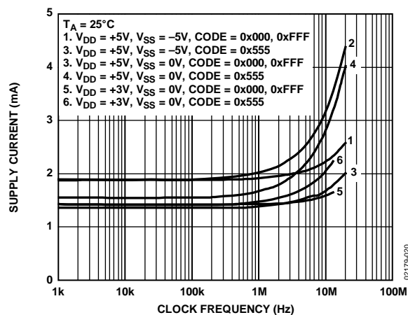
Figure 20. AD7398 Supply Current vs. Clock Frequency
