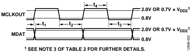
Figure 2. Data Timing
