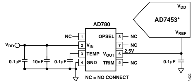
Figure 22. Typical V_{\text{REF}} Connection Diagram for V_{\text{DD}} = 5 V
