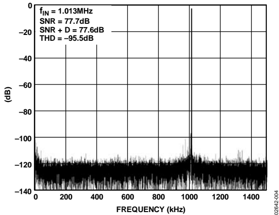
Figure 4. 64 k FFT Plot with 1 MHz Input Tone
