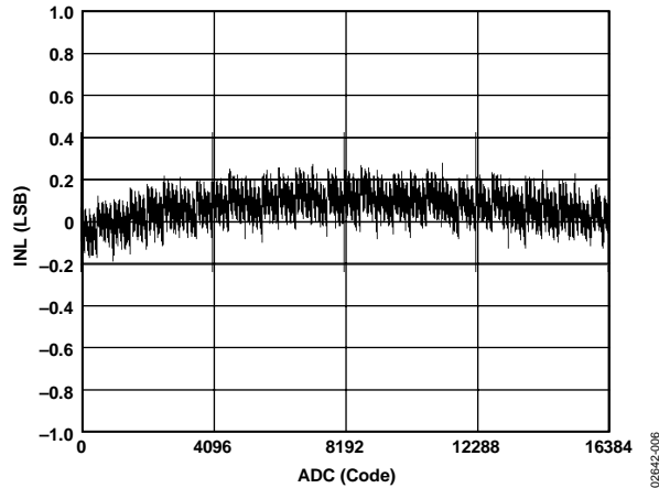
Figure 6. Typical INL
