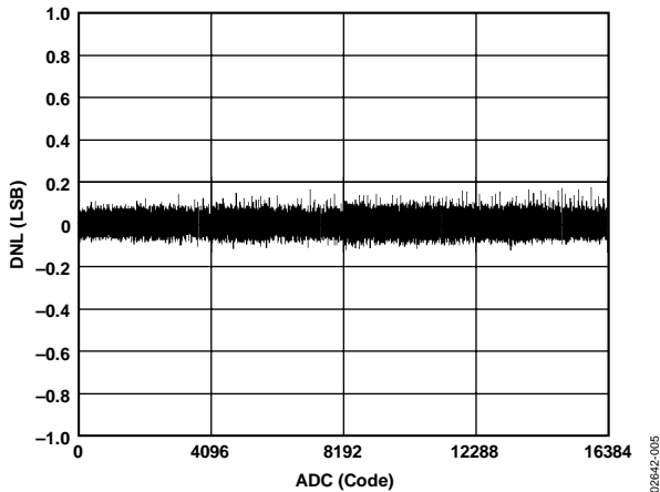
Figure 5. Typical DNL
