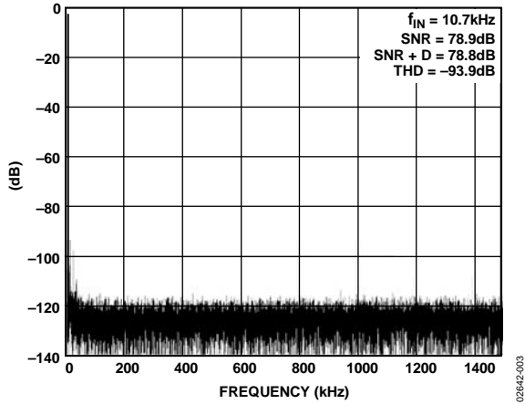
Figure 3. 64 k FFT Plot with 10 kHz Input Tone
