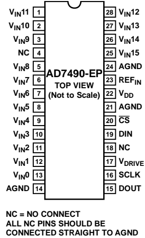
Figure 3. 28-Lead TSSOP Pin Configuration
