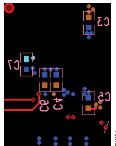
Figure 53. Bottom Layer Decoupling
