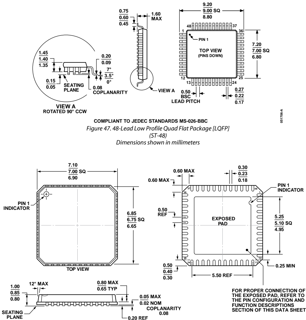
Figure 48. 48-Lead Lead Frame Chip Scale Package (LFCSP_VQ) 7 mm x 7 mm Body, Very Thin Quad (CP-48-1)
