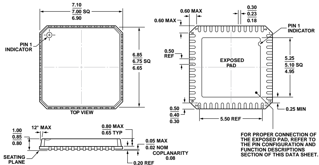
Figure 48. 48-Lead Lead Frame Chip Scale Package (LFCSP_VQ) 7 mm x 7 mm Body, Very Thin Quad (CP-48-1)
