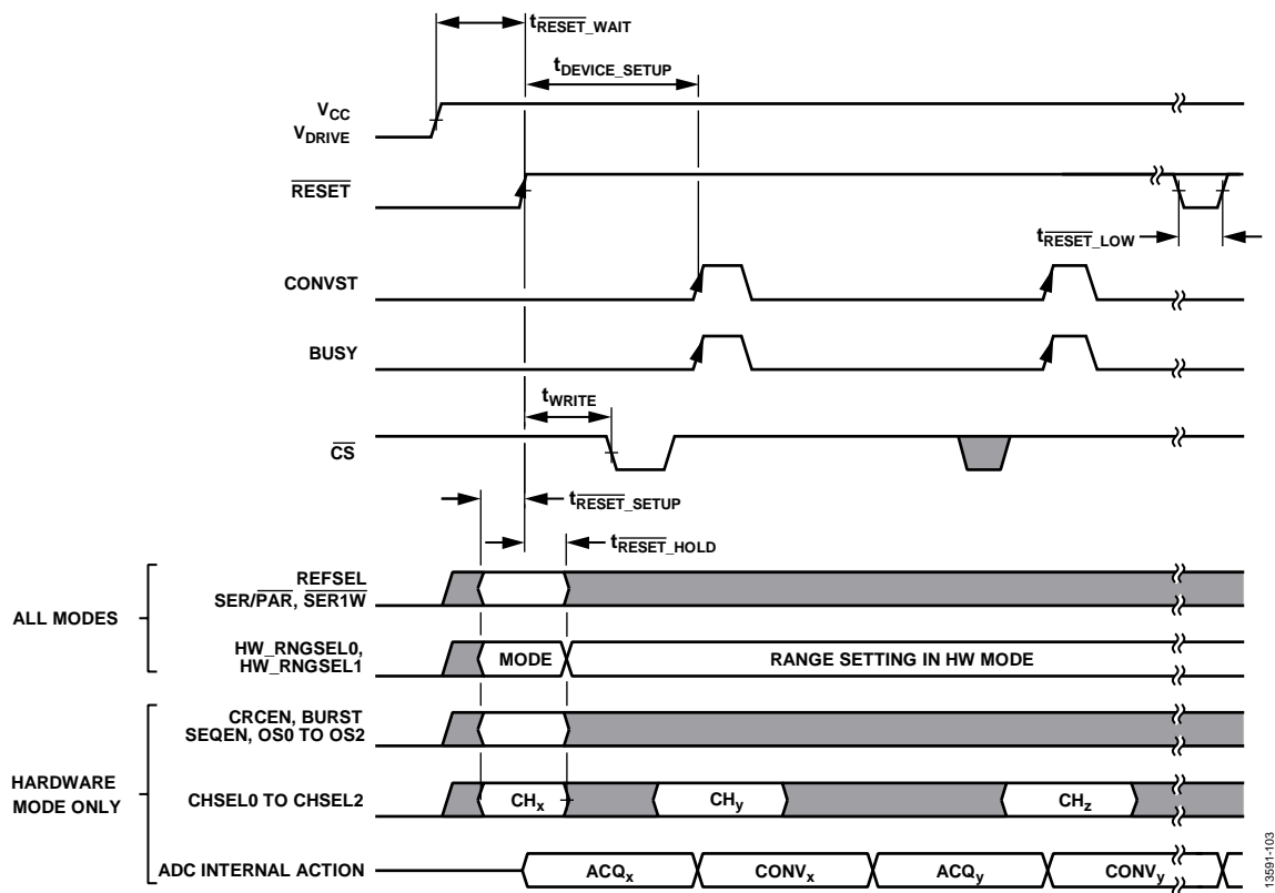
Figure 3. Reset Timing
