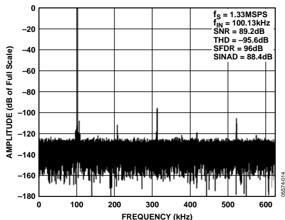
Figure 14. FFT 100 kHz
