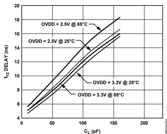
Figure 20. Typical Delay vs. Load Capacitance C_L
