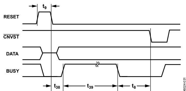
Figure 31. RESET Timing
