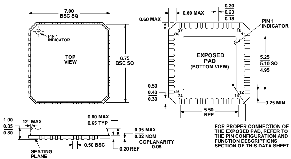
Figure 40. 48-Lead Lead Frame Chip Scale Package [LFCSP_VQ] 7 mm x 7 mm Body, Very Thin Quad (CP-48-1)
