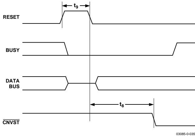
Figure 33. RESET Timing
