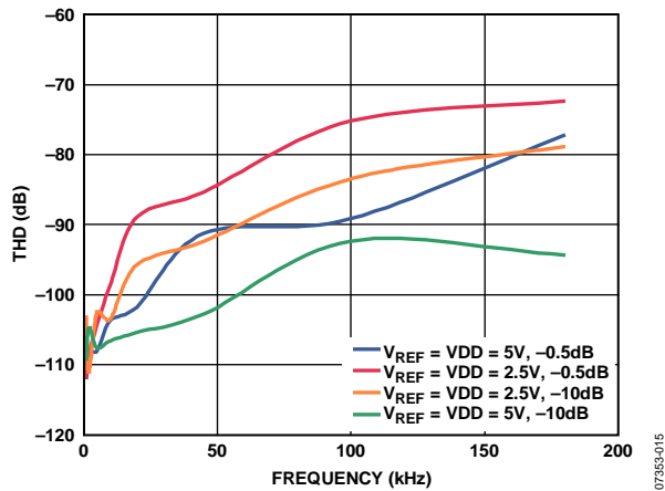
Figure 20. THD vs. Frequency
