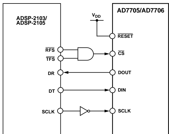
Figure 24. AD7705/AD7706-to-ADSP-2103/ADSP-2105 Interface
