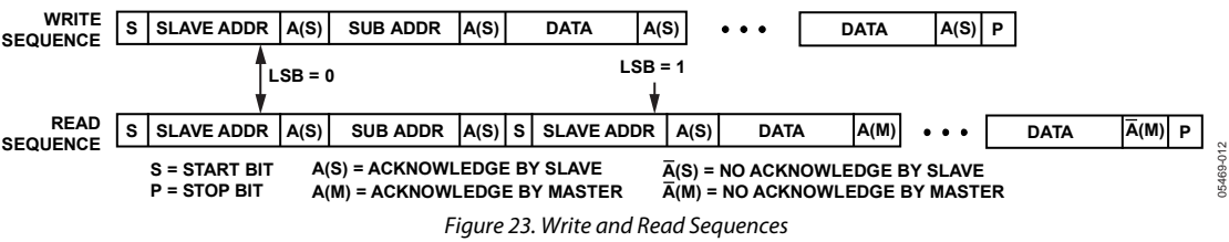
Figure 23. Write and Read Sequences
