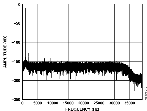
Figure 10. Low Power FFT, 1 kHz, -0.6\text{ dB} Input Tone, 256 \times Decimation
