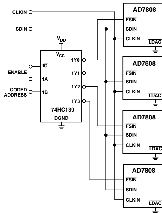
Figure 42. Decoding Multiple AD7808s Using the \overline{FSIN} Pin
