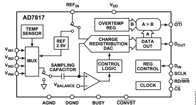
Figure 1. AD7817 Functional Block Diagram
