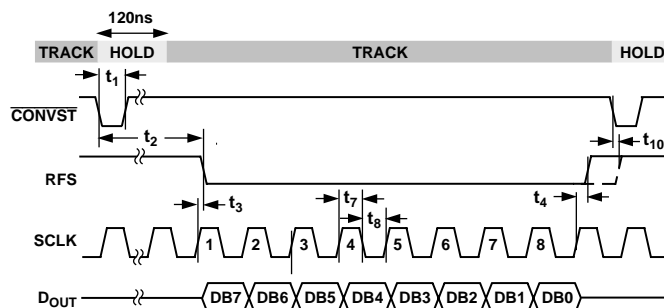
Figure 4. Track-and-Hold Timing
