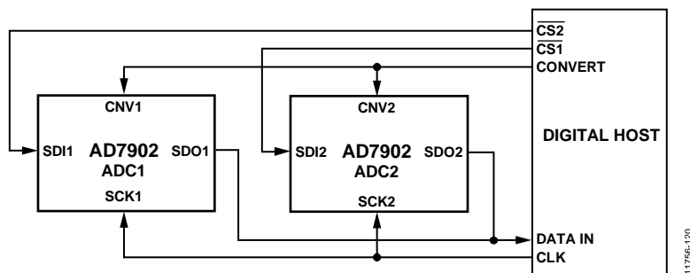
Figure 42. \overline{CS} Mode, 4-Wire Interface Without a Busy Indicator Connection Diagram
