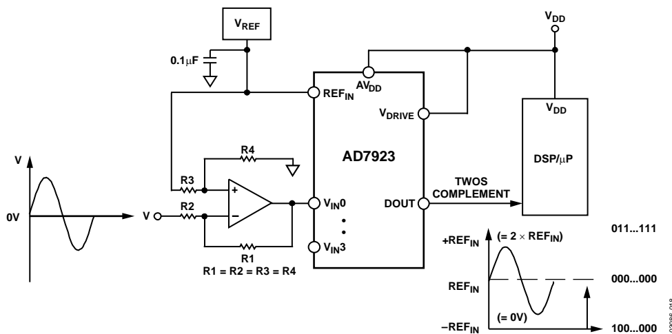
Figure 18. Handling Bipolar Signals
