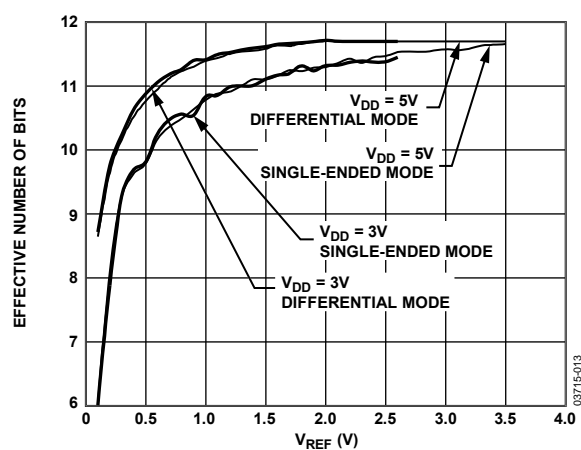
Figure 11. AD7938 ENOB vs. V_{REF}
