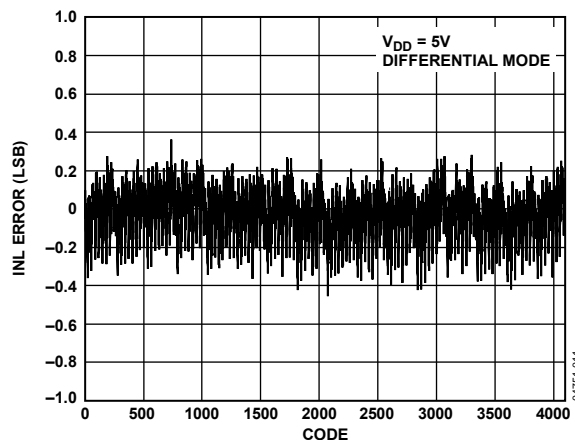
Figure 9. AD7938-6 Typical INL @ V_{DD} = 5V
