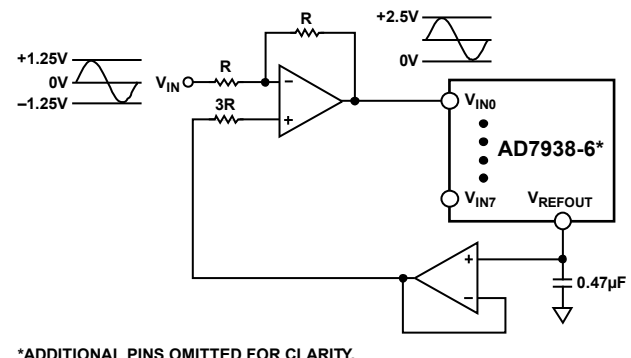
Figure 24. Single-Ended Mode Connection Diagram
