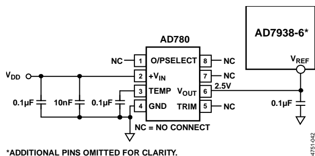
Figure 35. Typical V_{REF} Connection Diagram
