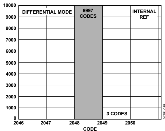
Figure 13. AD7938-6 Histogram of Codes for 10,000 Samples @ V_{DD} = 5\text{ V} with Internal Reference
