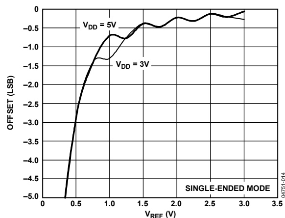
Figure 12. AD7938-6 Offset vs. V_{REF}
