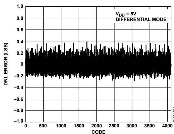
Figure 8. AD7938-6 Typical DNL @ V_{DD} = 5V
