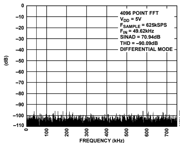
Figure 7. AD7938-6 FFT @ V_{DD} = 5V
