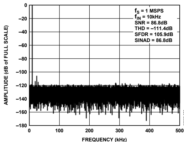
Figure 11. FFT Plot, REF = 2.5\text{ V}
