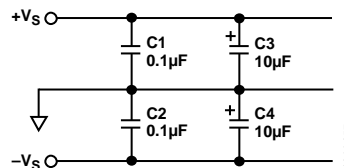
Figure 58. Supply Bypassing
