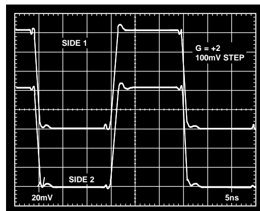
Figure 9. 1 V Step Response, G = +2
