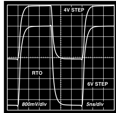
TPC 5. 1 Step Response; G = -2 , V_S = \pm 5 \text{ V}
