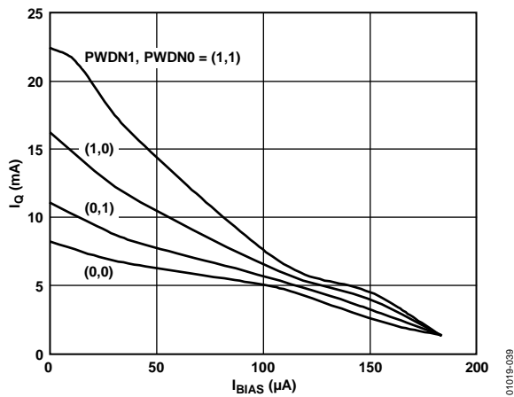
Figure 37. I_Q vs. I_{BIAS} Current; V_S = \pm 12 V
