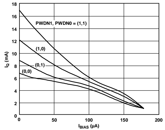
Figure 38. I_Q vs. I_{BIAS} Current; V_S = \pm 6 V
