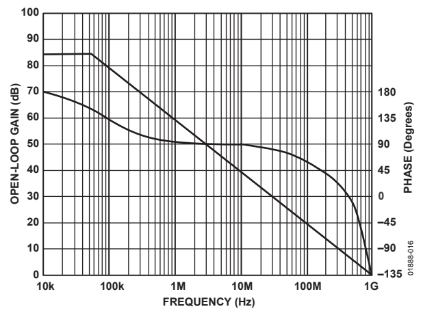
Figure 16. Open-Loop Gain and Phase vs. Frequency, R_G = 100\text{ }\Omega , R_F = 1\text{ k}\Omega , R_O = 976\text{ }\Omega , R_D = 53.6\text{ }\Omega , C_C = 0\text{ pF} (See Figure 50)
