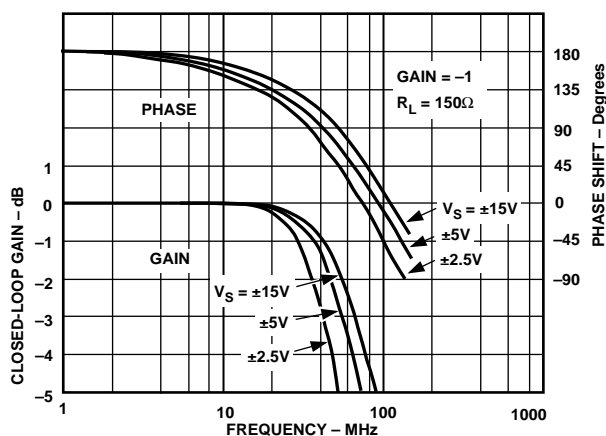
Figure 33. Closed-Loop Gain and Phase vs. Frequency G = -1 , R_L = 150 \Omega , R_F = 681 \Omega for \pm 15 \text{ V} , 620 \Omega for \pm 5 \text{ V} and \pm 2.5 \text{ V}
