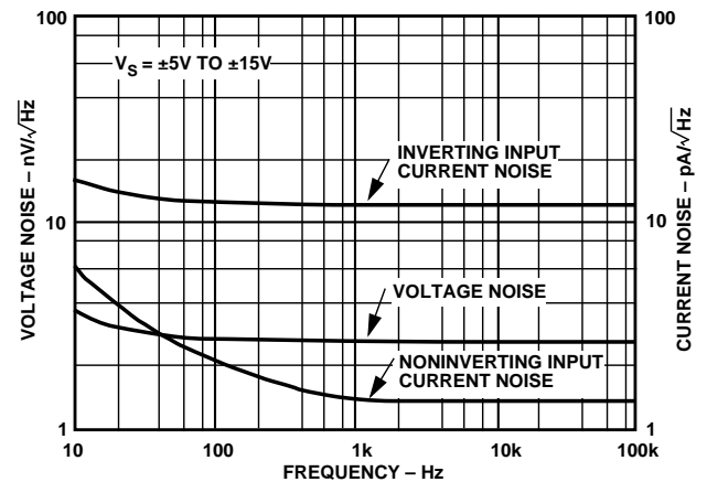
Figure 12. Input Voltage and Current Noise vs. Frequency
