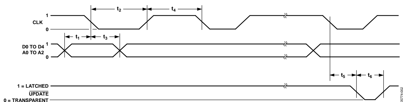
Figure 2. Timing Diagram
