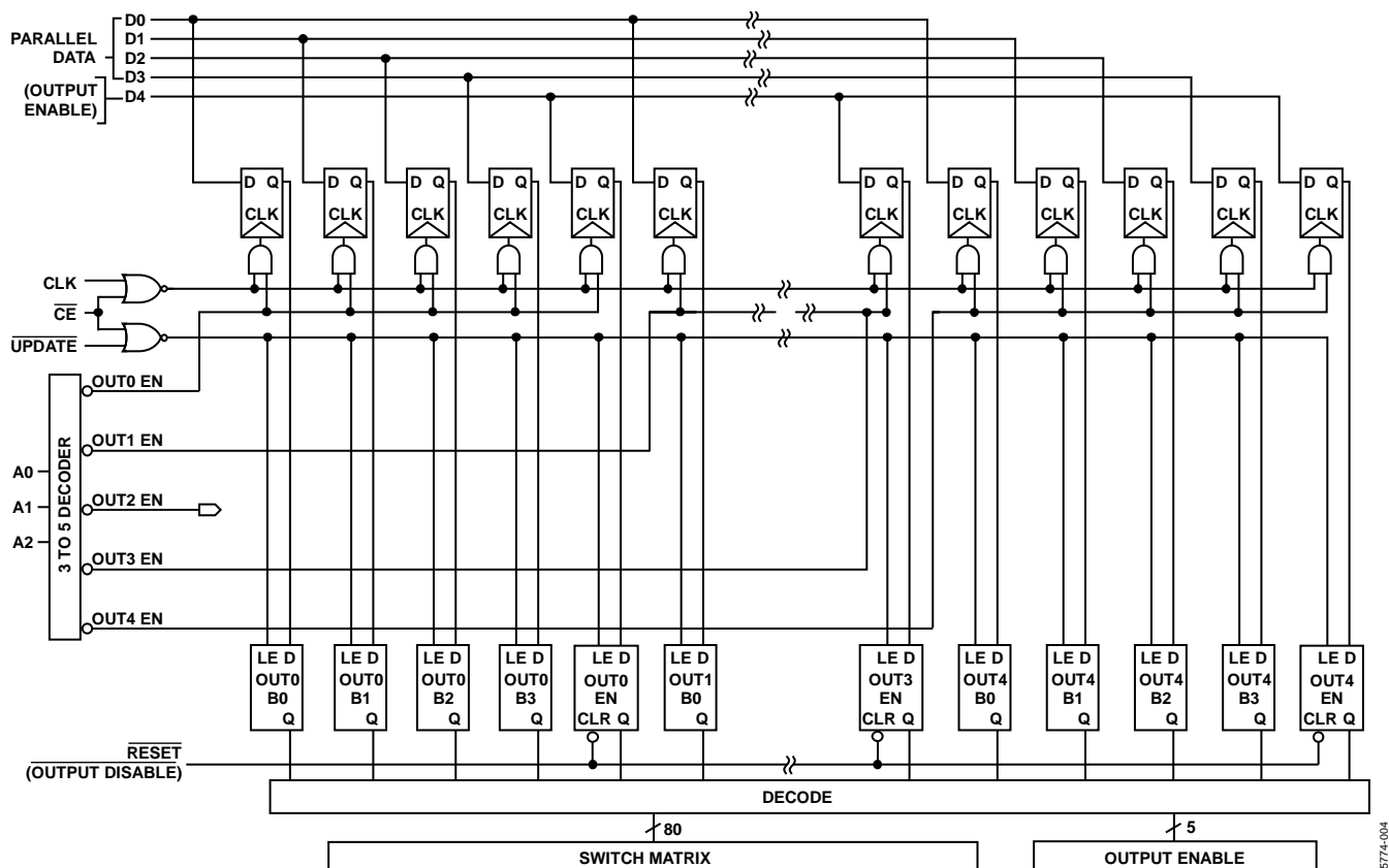
Figure 4. Logic Diagram
