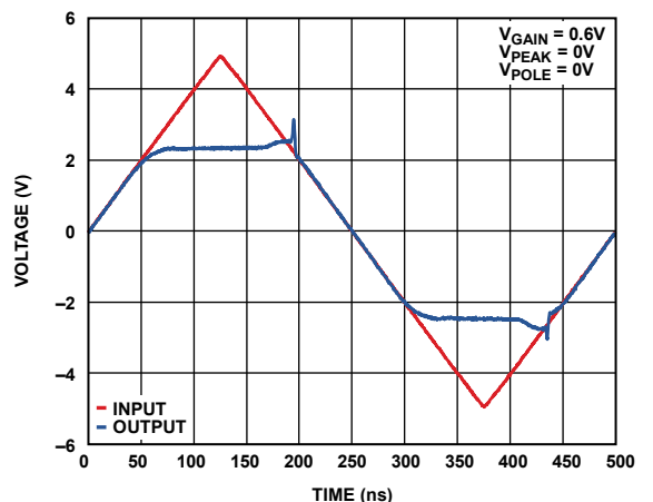
Figure 9. Overdrive Recovery
