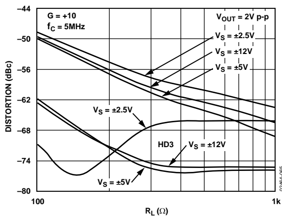
Figure 64. AD8129 Harmonic Distortion vs. Load Resistance
