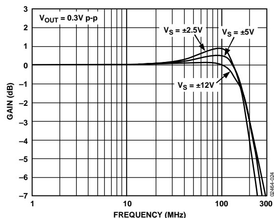
Figure 23. AD8129 Frequency Response vs. Supply, V_{OUT} = 0.3\text{ V p-p}
