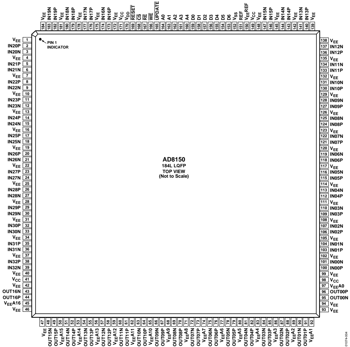
Figure 4. Pin Configuration
