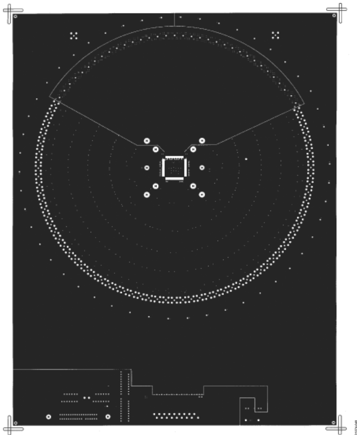
Figure 49. INT1 ( V_{EE} )
