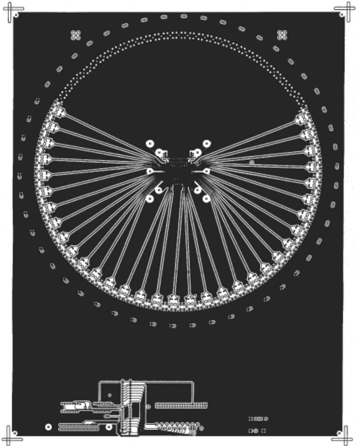
Figure 44. Circuit Side
