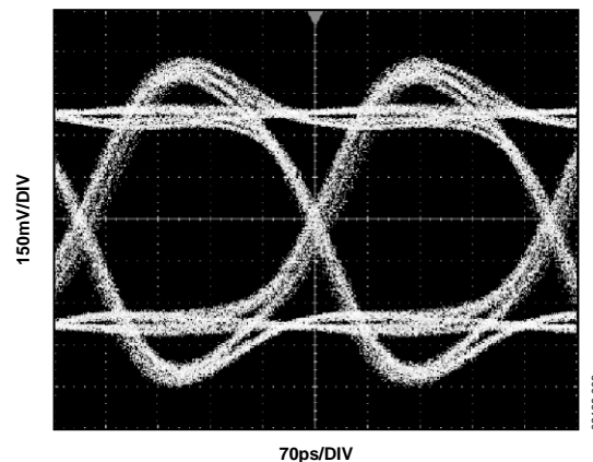
Figure 2. Eye Pattern, 3.2 Gbps, PRBS 23
