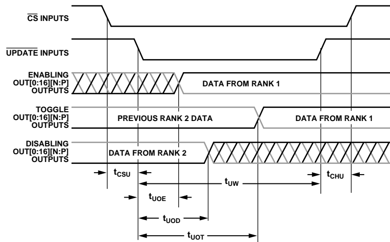
Figure 28. Second Rank Update Cycle
