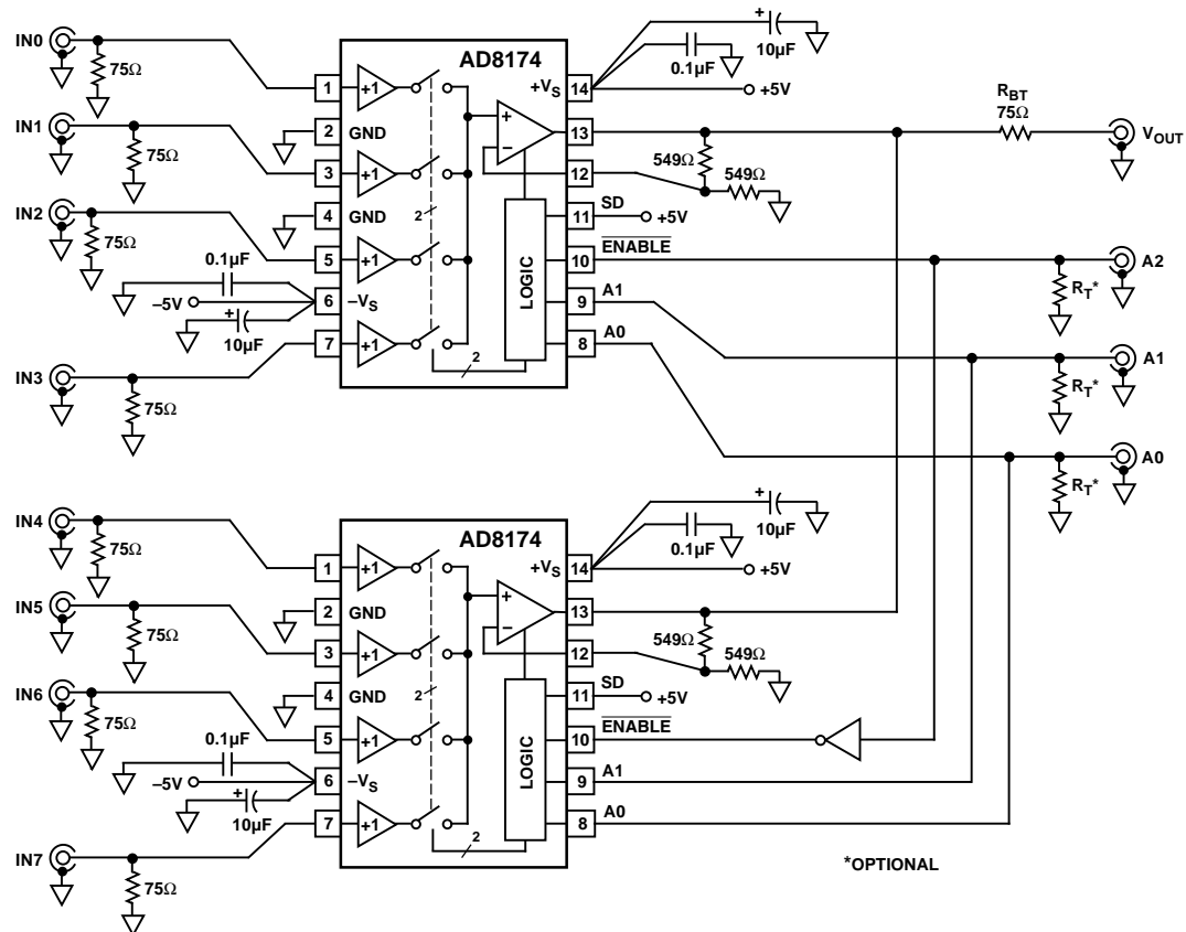
Figure 26. 8-to-1 Multiplexer
