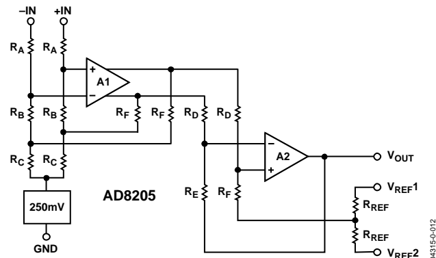
Figure 13. Simplified Schematic
