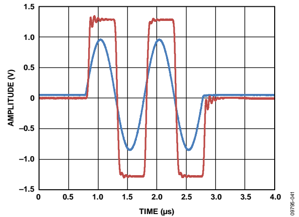
Figure 19. Overdrive Recovery
