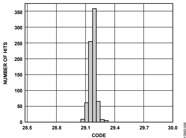
Figure 6. Gain Histogram (Gain = 29 dB)
