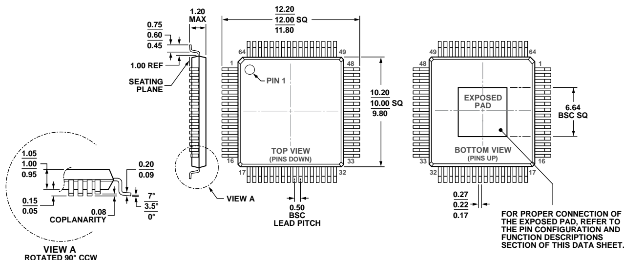
Figure 25. 64-Lead Thin Quad Flat Package, Exposed Pad [TQFP_EP] (SV-64-5) Dimensions shown in millimeters
