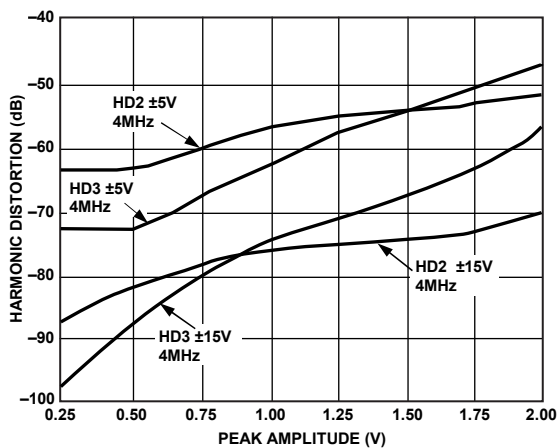
Figure 16. Harmonic Distortion vs. Peak Amplitude, Frequency = 4 MHz
