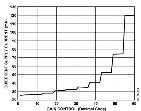
Figure 18. Supply Current vs. Gain Control
