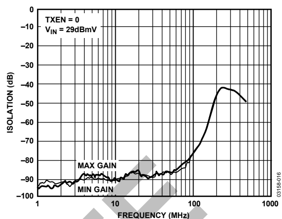
Figure 16. Isolation in Transmit Disable Mode vs. Frequency
