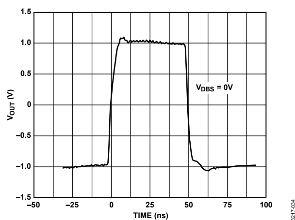
Figure 33. Full-Scale Transient Response, V_{DBS} = 0\text{V}
