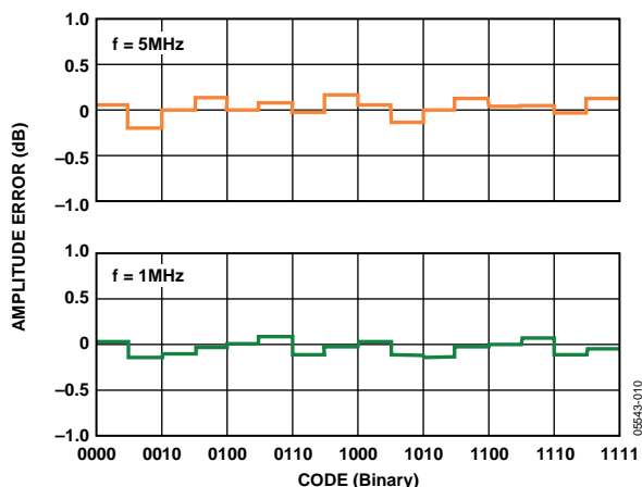
Figure 10. Amplitude Error of Channel 2 with Respect to Channel 1 vs. Code at 1 MHz and 5 MHz
