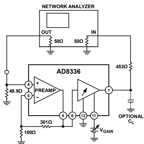
Figure 57. Frequency Response
