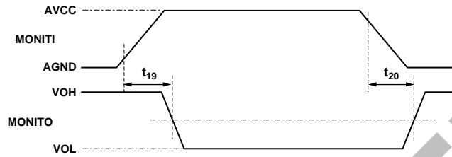
Figure 12. Level Shifting Edge Detector Timing
