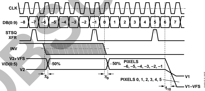
Figure 7. Output Timing ( R/L = \text{Low} , E/O = \text{High} )
